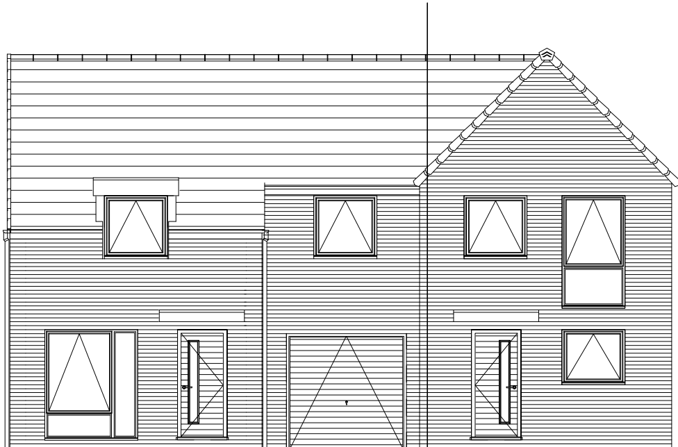
340 301 FRONT ELEVATION
