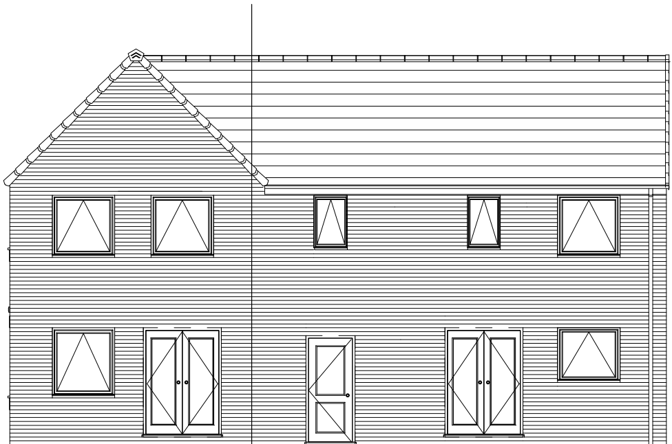
301 340 REAR ELEVATION
