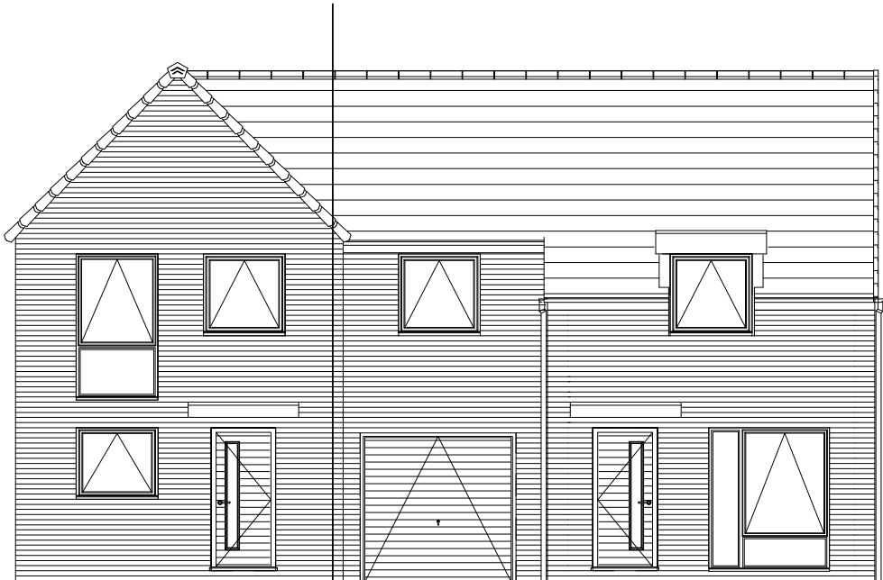
301 340 FRONT ELEVATION
