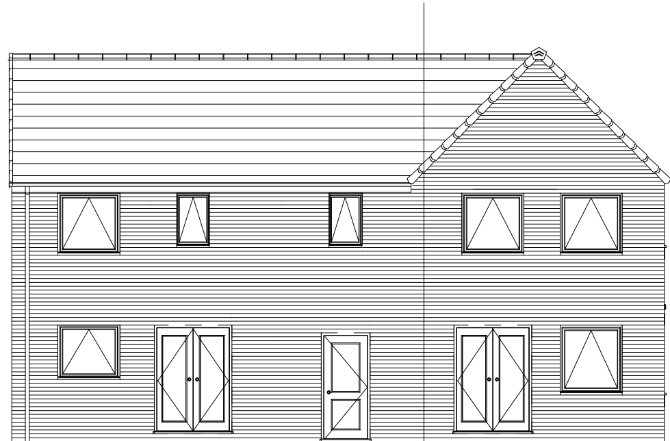
340 301 REAR ELEVATION
