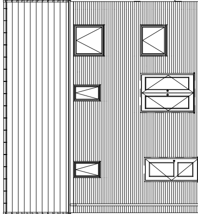
REAR ELEVATION
