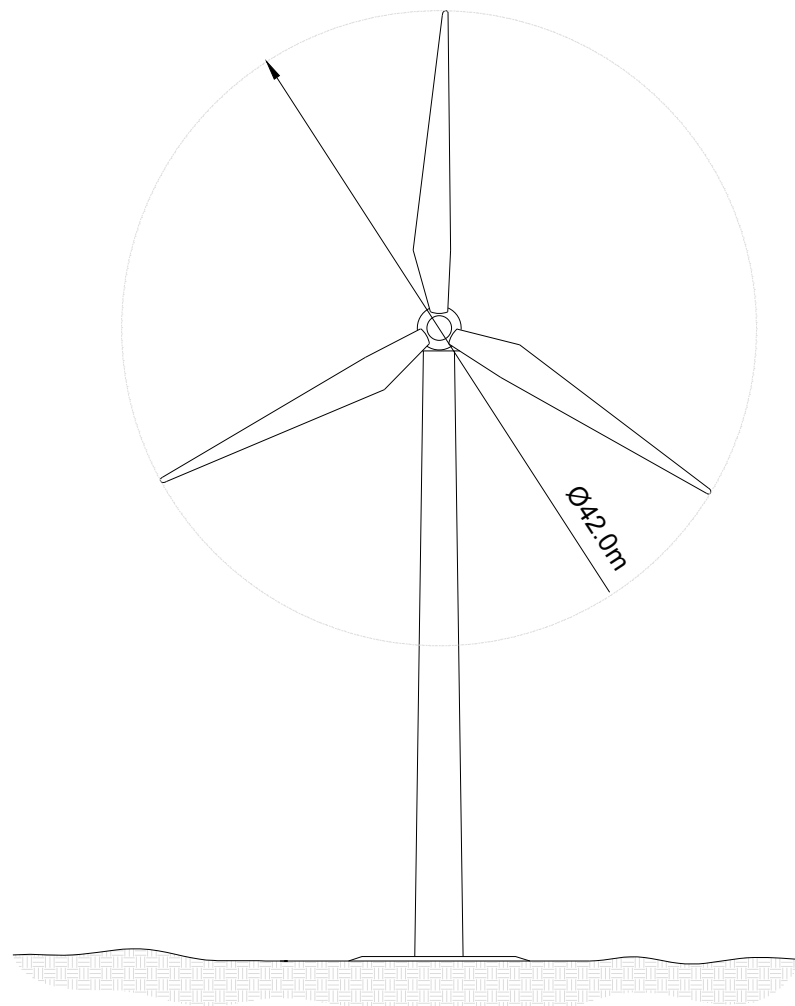
FRONT ELEVATION SCALE = 1:500
