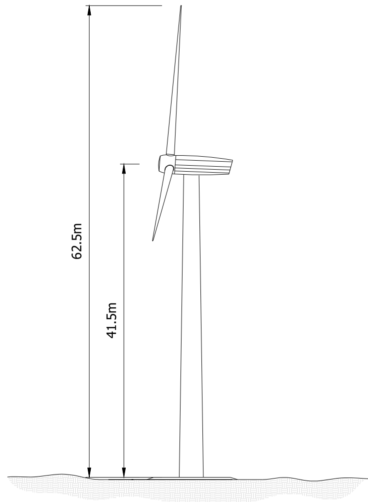
SIDE ELEVATION SCALE = 1:500
