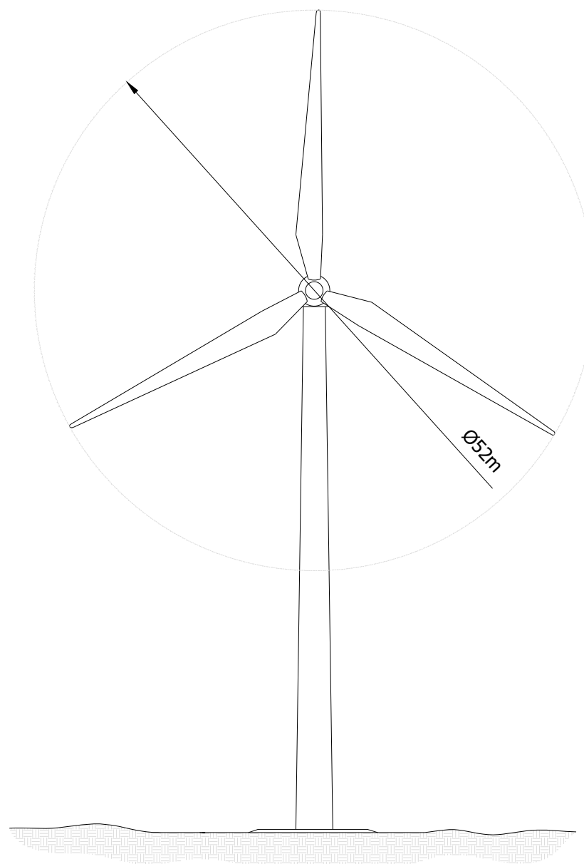
FRONT ELEVATION SCALE = 1:500
