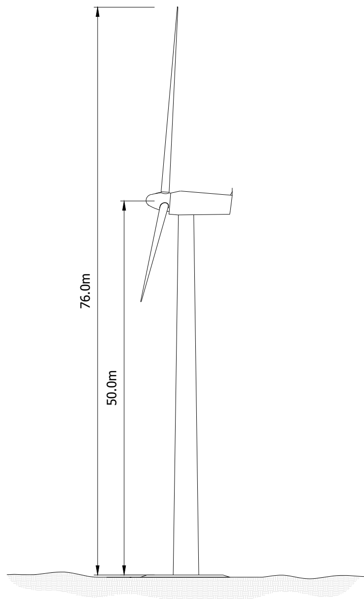
SIDE ELEVATION SCALE = 1:500
