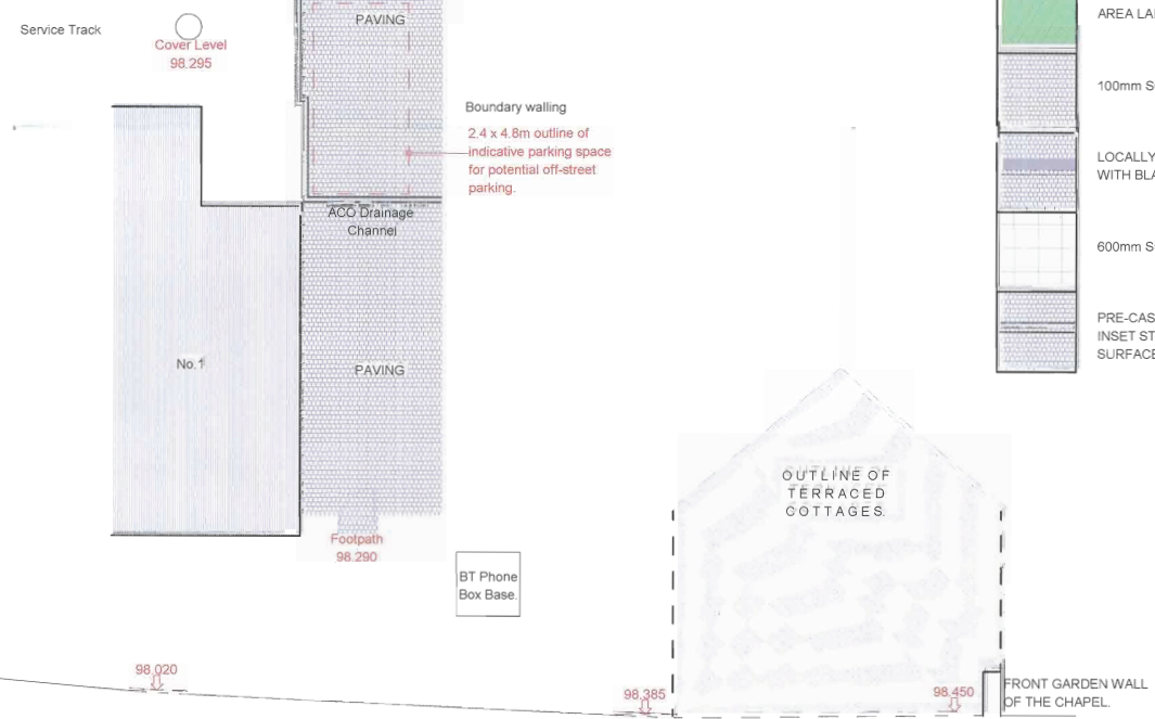
INDICATIVE SECTION OF EXISTING SITE LEVELS.
