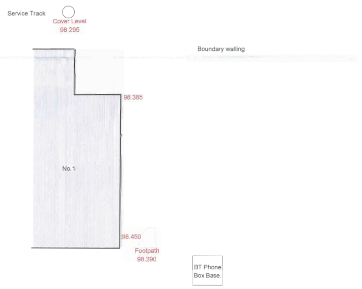
EXISTING SITE PLAN & SPOT LEVEL SURVEY.
