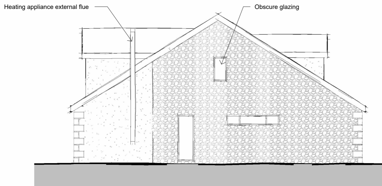
Side Elevation 02 1 : 100
