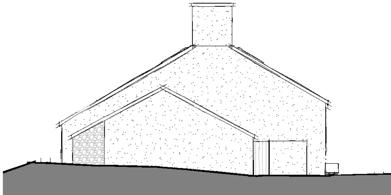
Side Elevation 02 1 : 100
