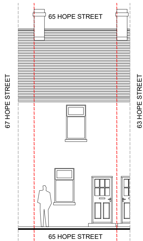
1 EXISTING FRONT ELEVATION Scale 1:100
