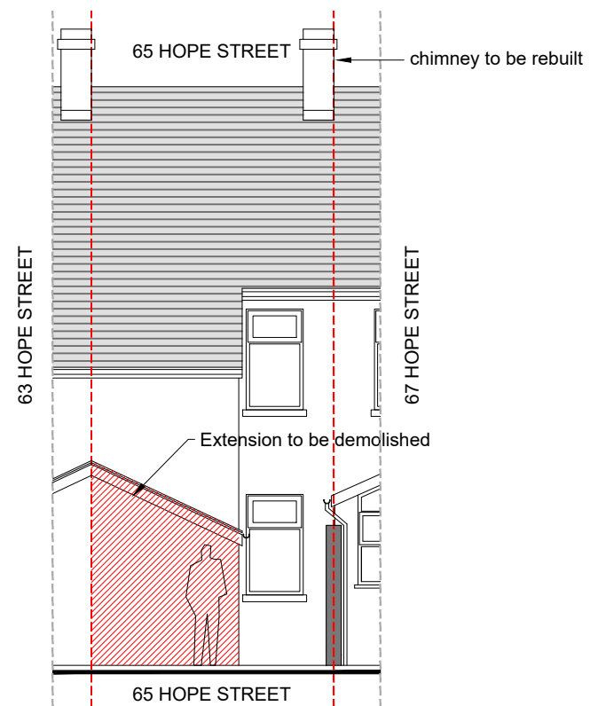
2 EXISTING REAR ELEVATION Scale 1:100
