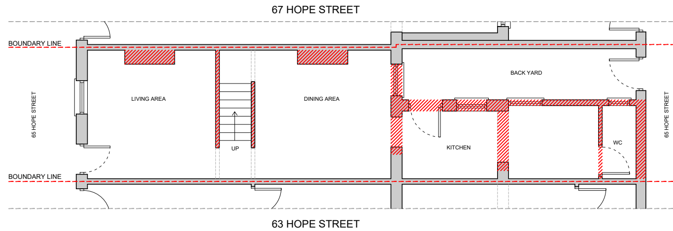
1 EXISTING GROUND FLOOR PLAN Scale 1:100
