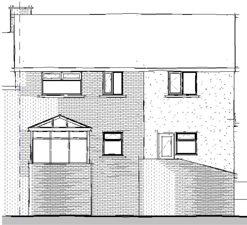
Rear Elevation 1 : 100
