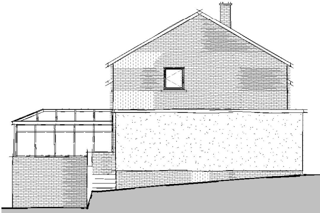
Side Elevation 02 1 : 100
