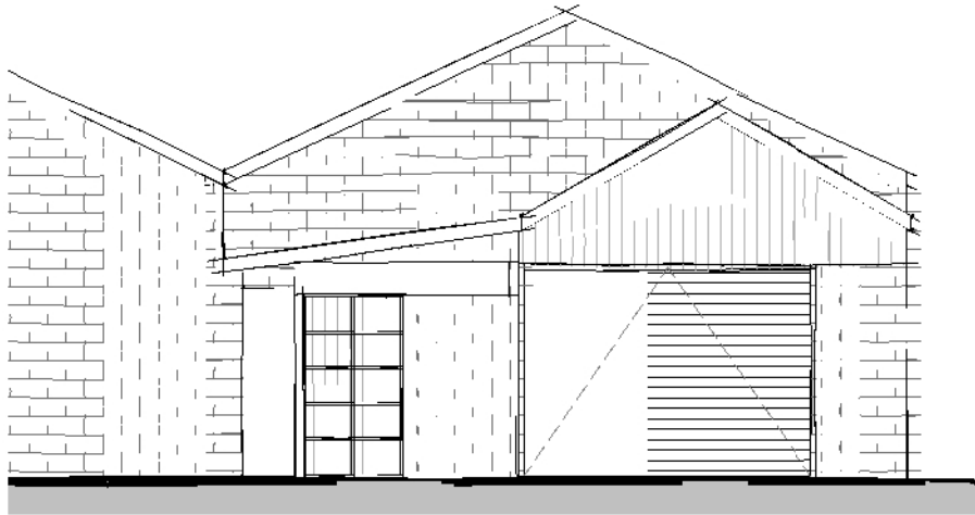
Front Elevation 1 : 100
