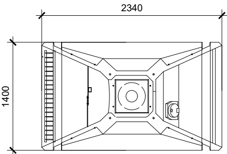
PROPOSED FOUNDATION PLAN
