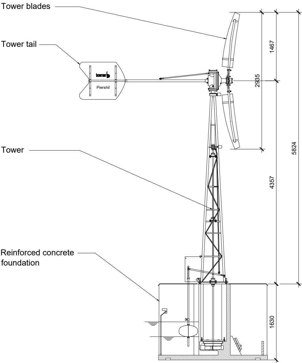
PROPOSED ELEVATION
