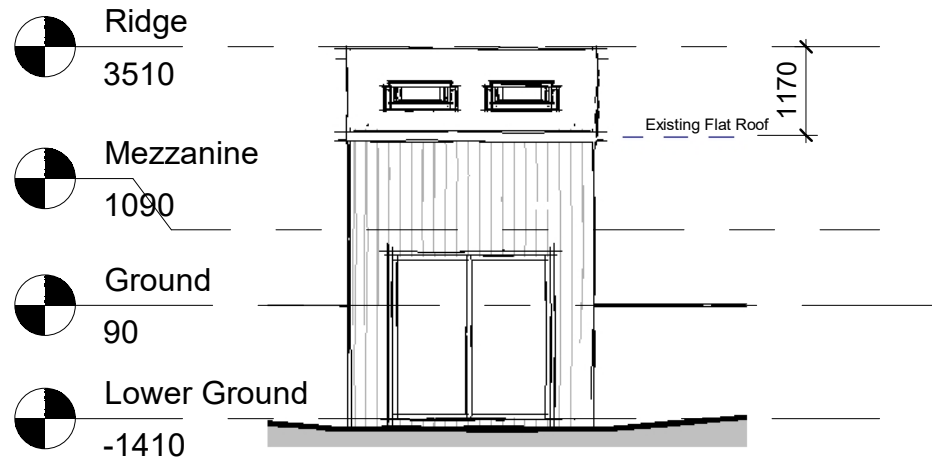
Rear Elevation
