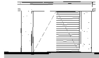
Front Elevation 1 : 100
