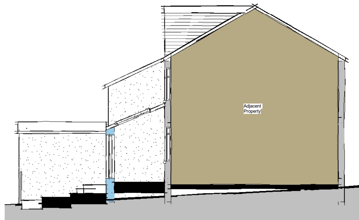
Side Elevation 02
