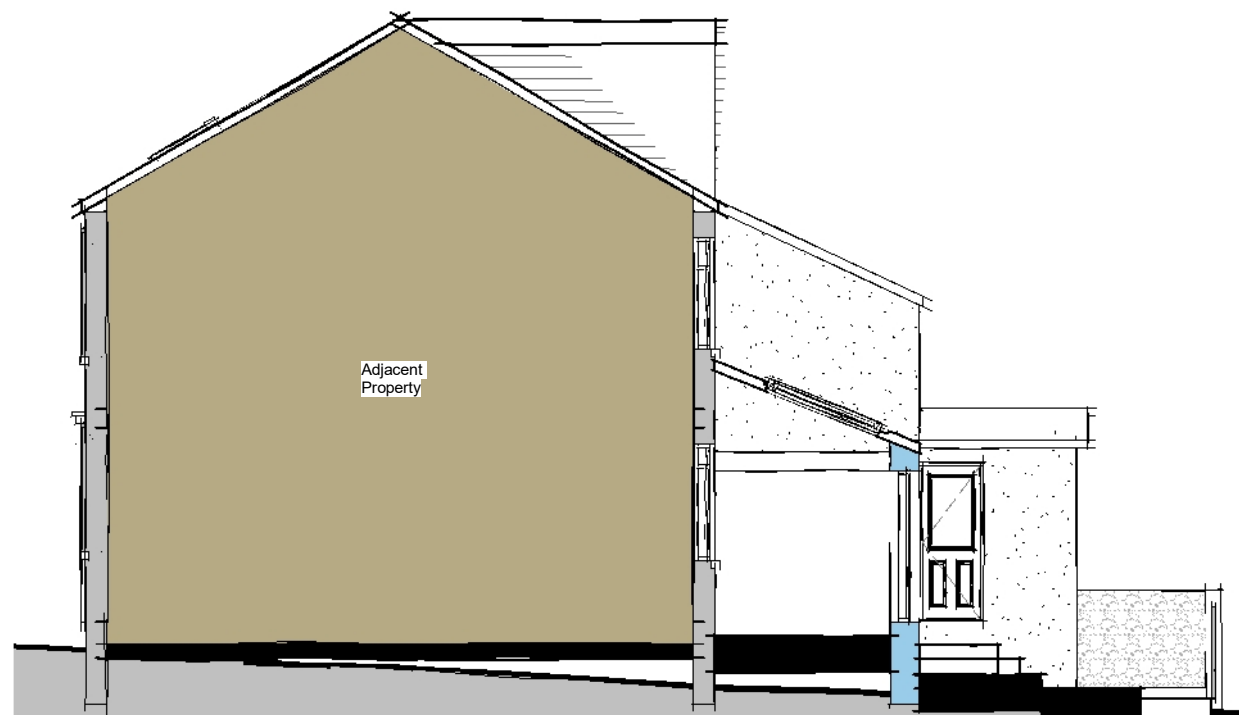
Side Elevation 01
