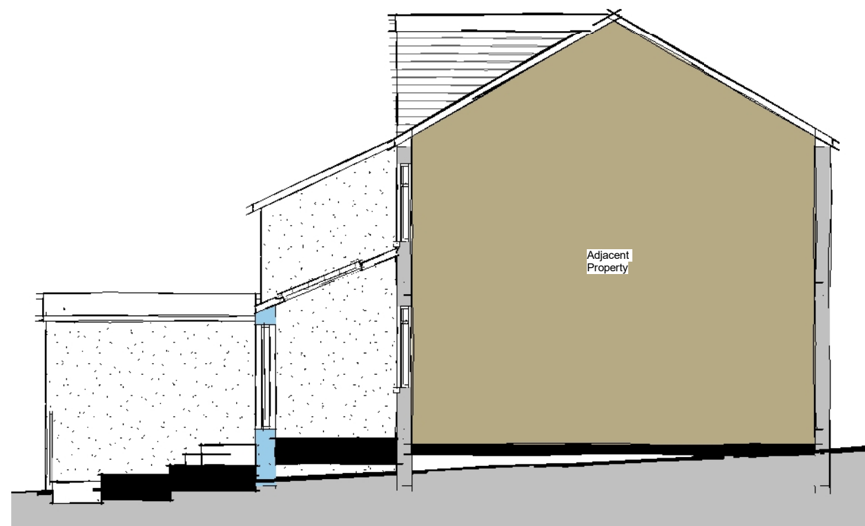
Side Elevation 02
