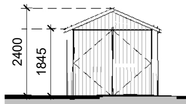
Front Elevation 1 : 100
