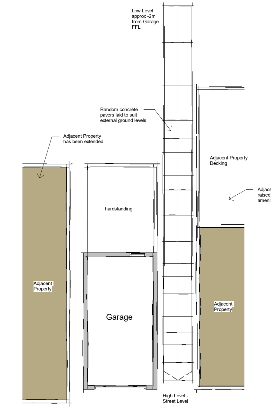
Ground 1 : 100
