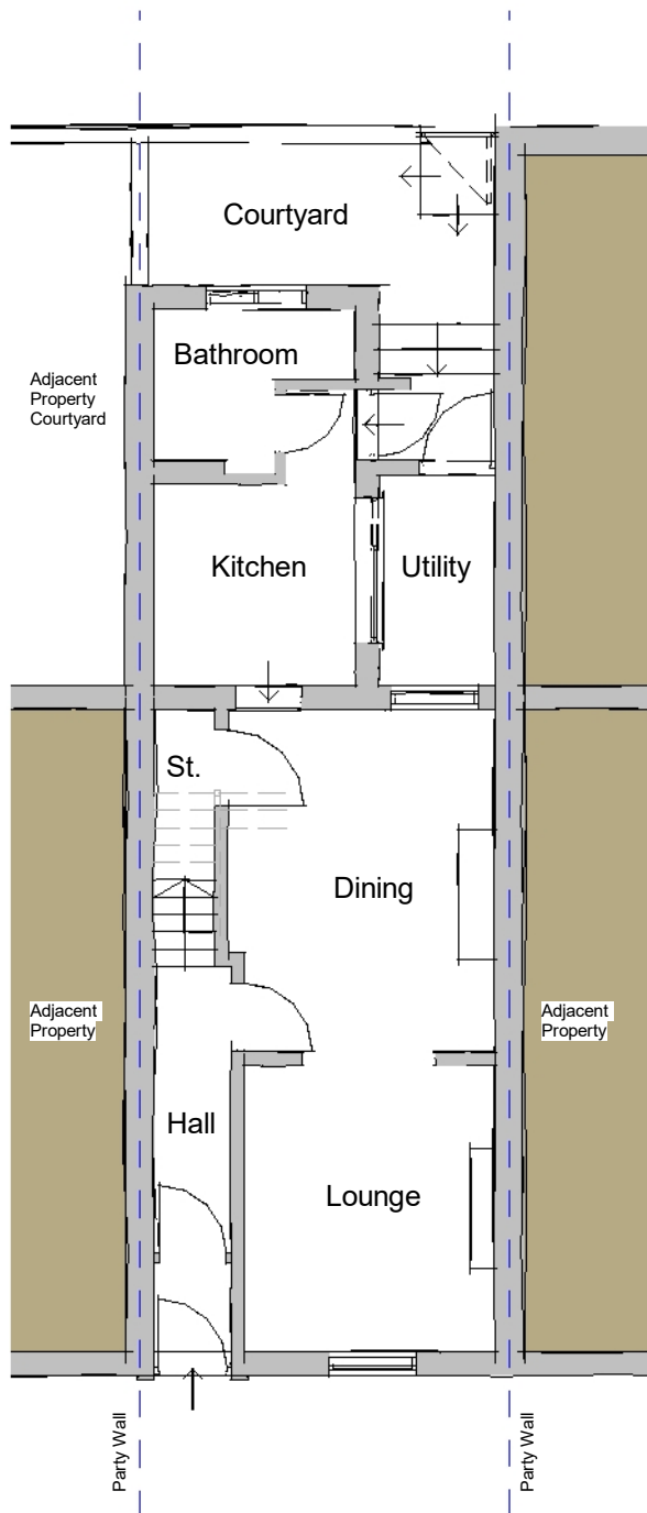
Ground 1 : 100
