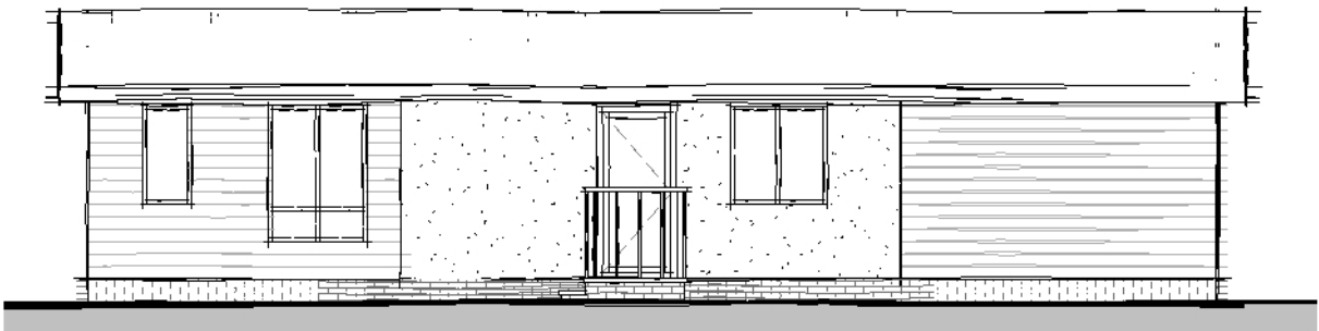
Rear Elevation 1 : 100
