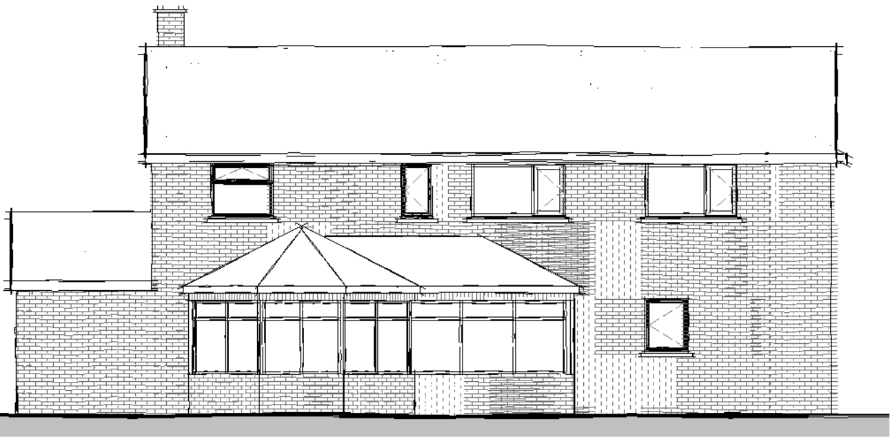
Rear Elevation 1 : 100
