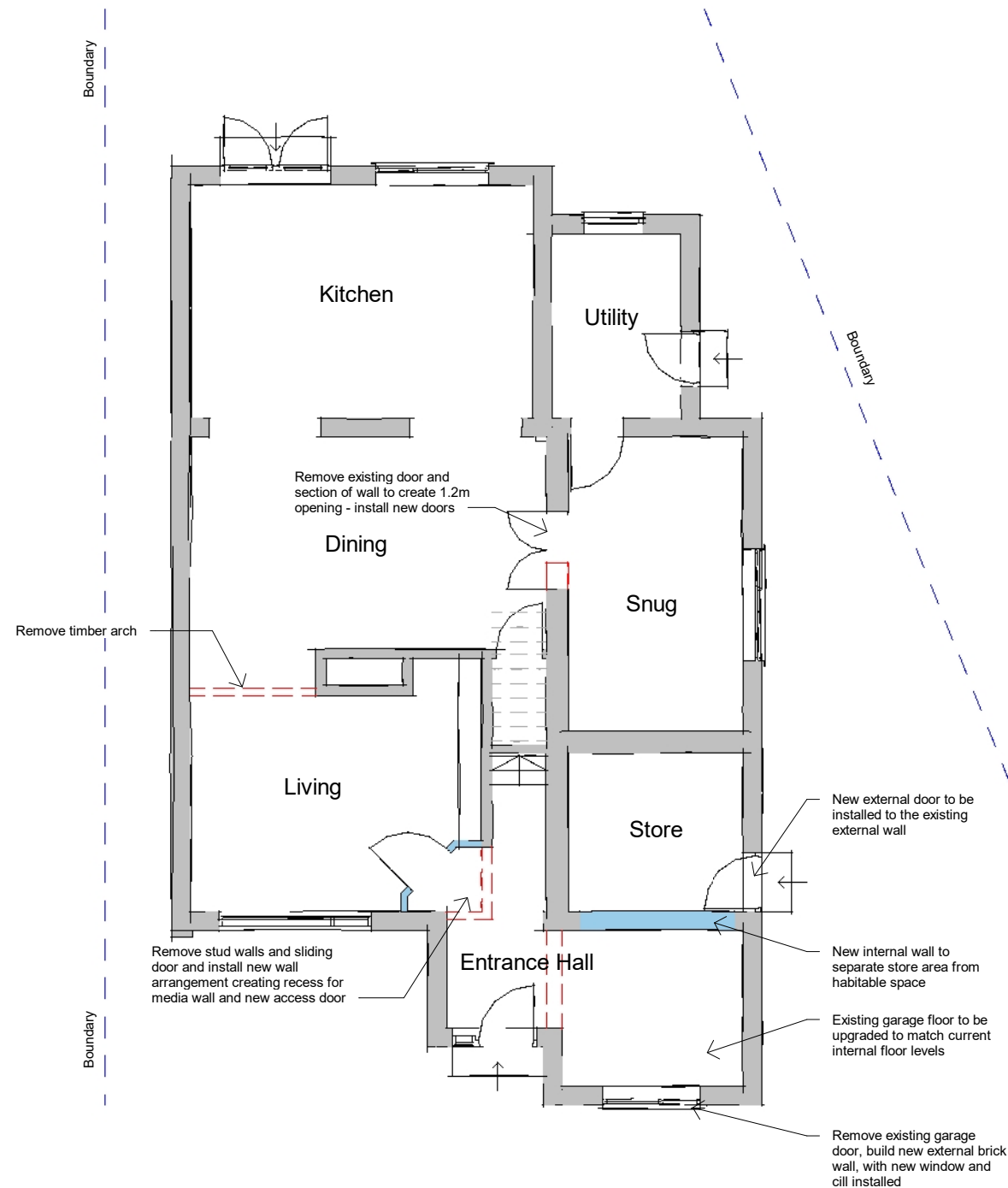
Ground 1 : 100
