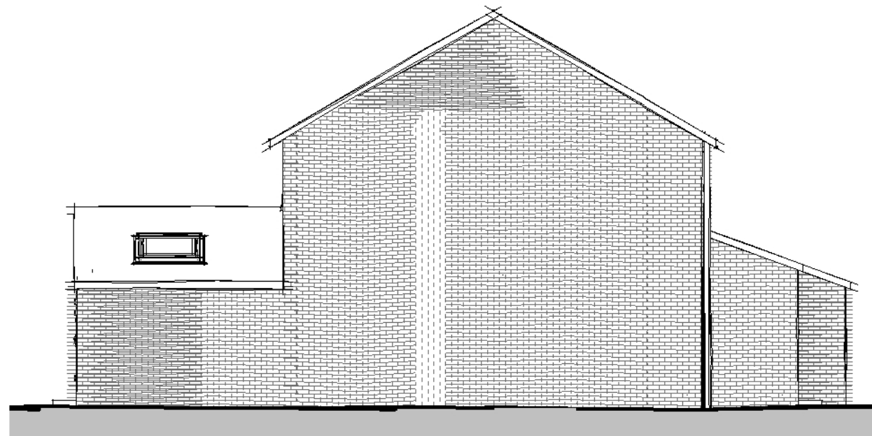
Side Elevation 02 1 : 100
