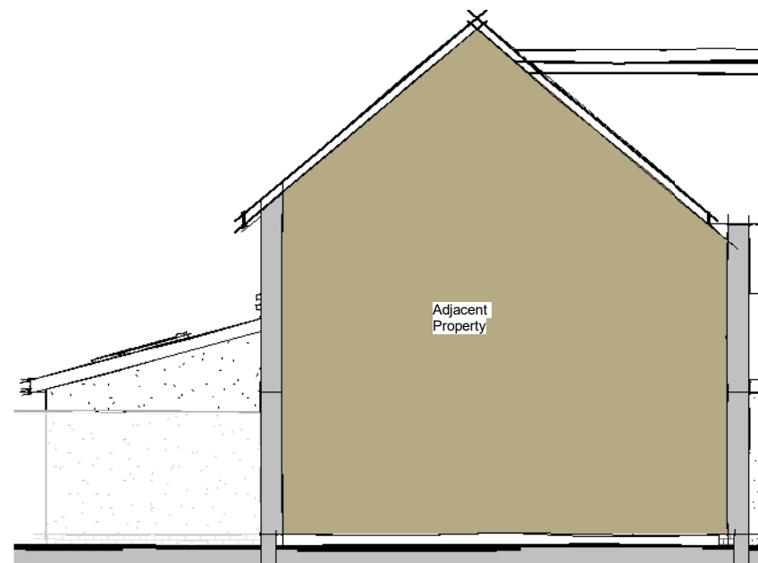
Side Elevation 02
