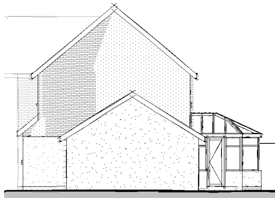
Side Elevation 01
