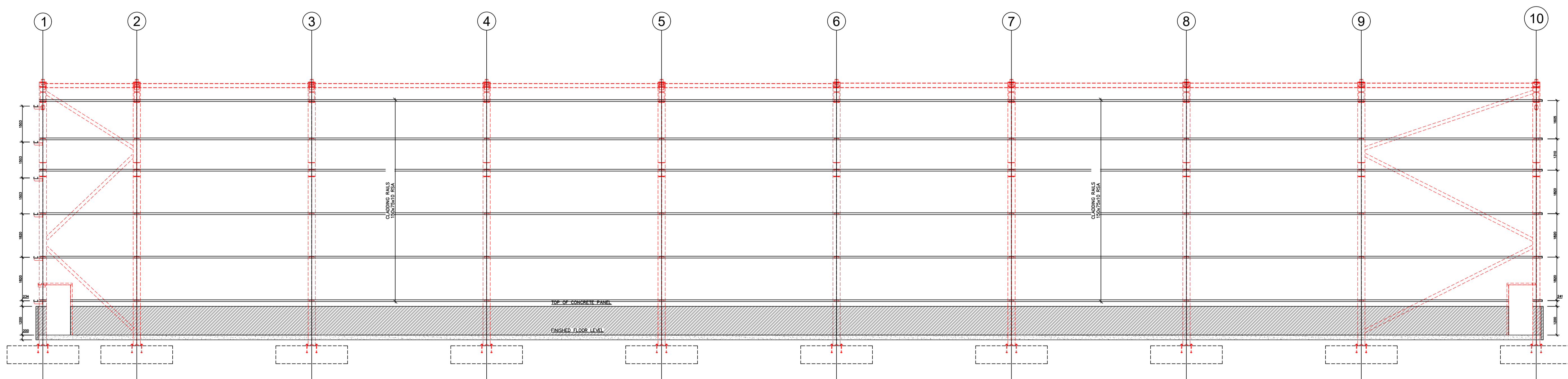
SECONDARY STEEL ELEVATION – GRIDLINE E SCALE 1:50
