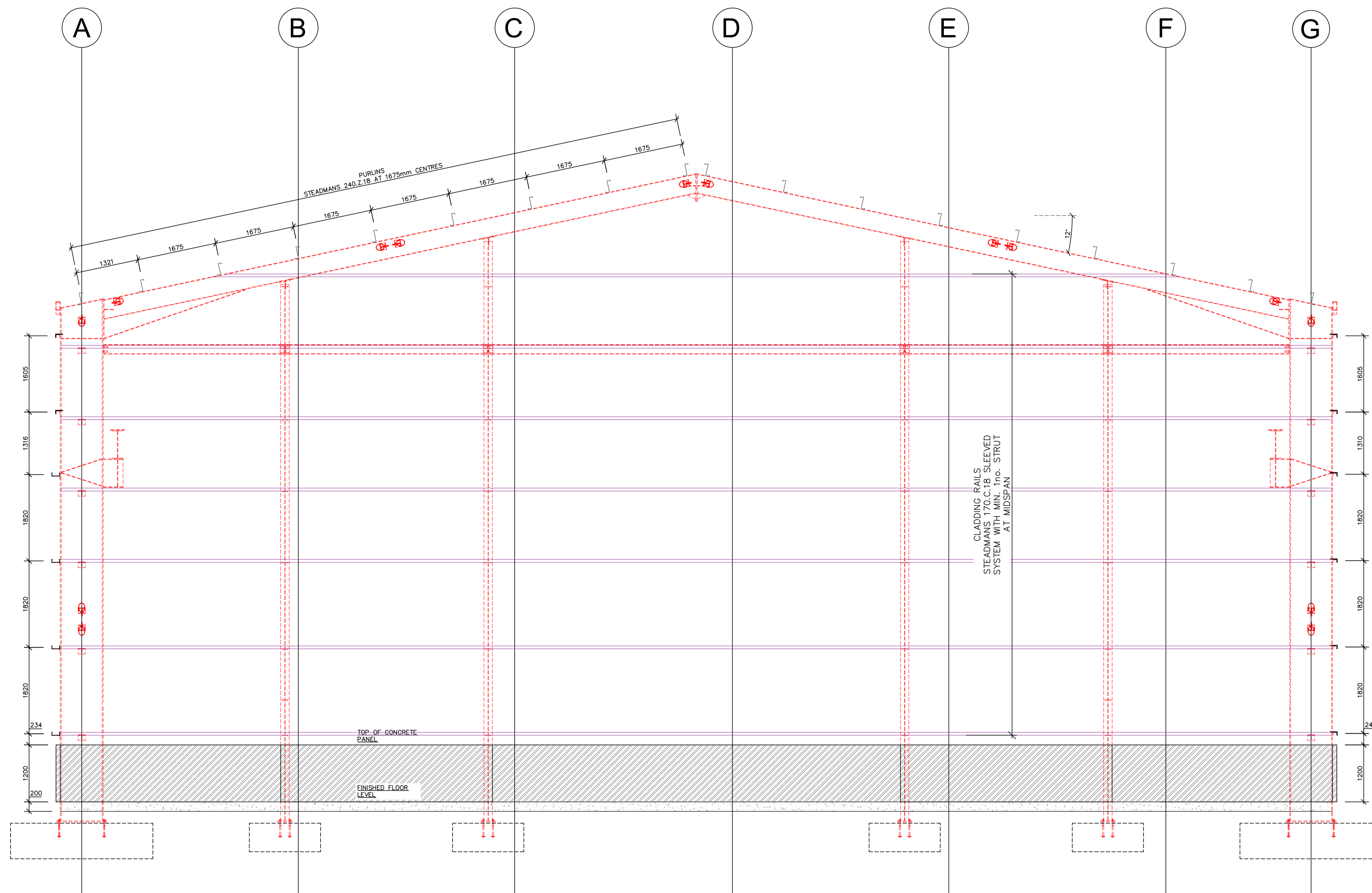
SECONDARY STEEL ELEVATION – GRIDLINE 1 SCALE 1:35
