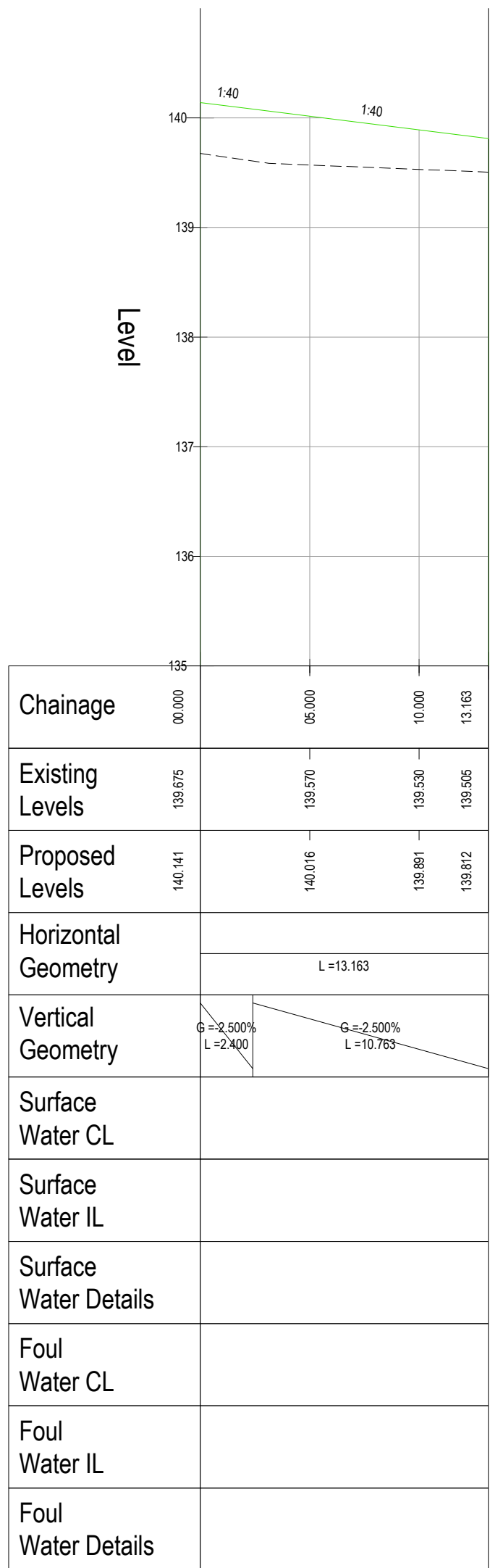
ROAD 17 TH - LONGSECTION SCALE: H 1:250, V 1:50. DATUM: 135.000
