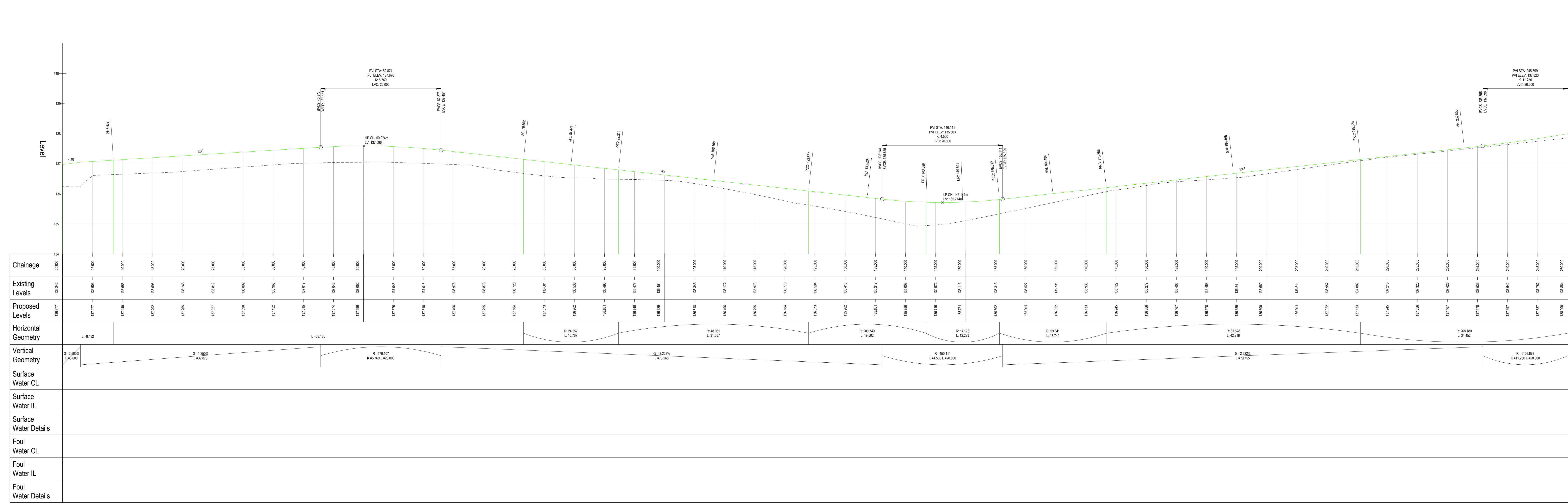
ROAD 15 - LONGSECTION CH 0-250 SCALE: H 1:250, V 1:50. DATUM: 134.000
