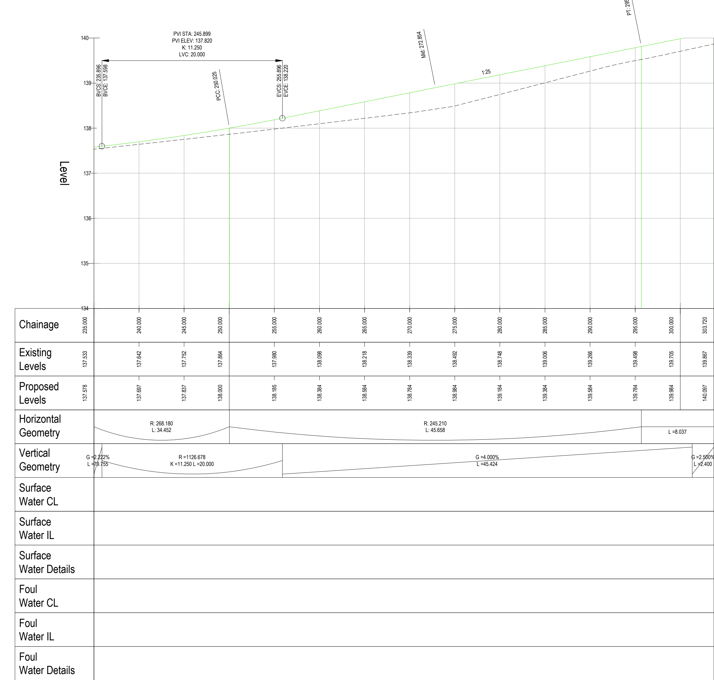
ROAD 15 - LONGSECTION CH 235-ROAD END SCALE: H 1:250, V 1:50. DATUM: 134.000
