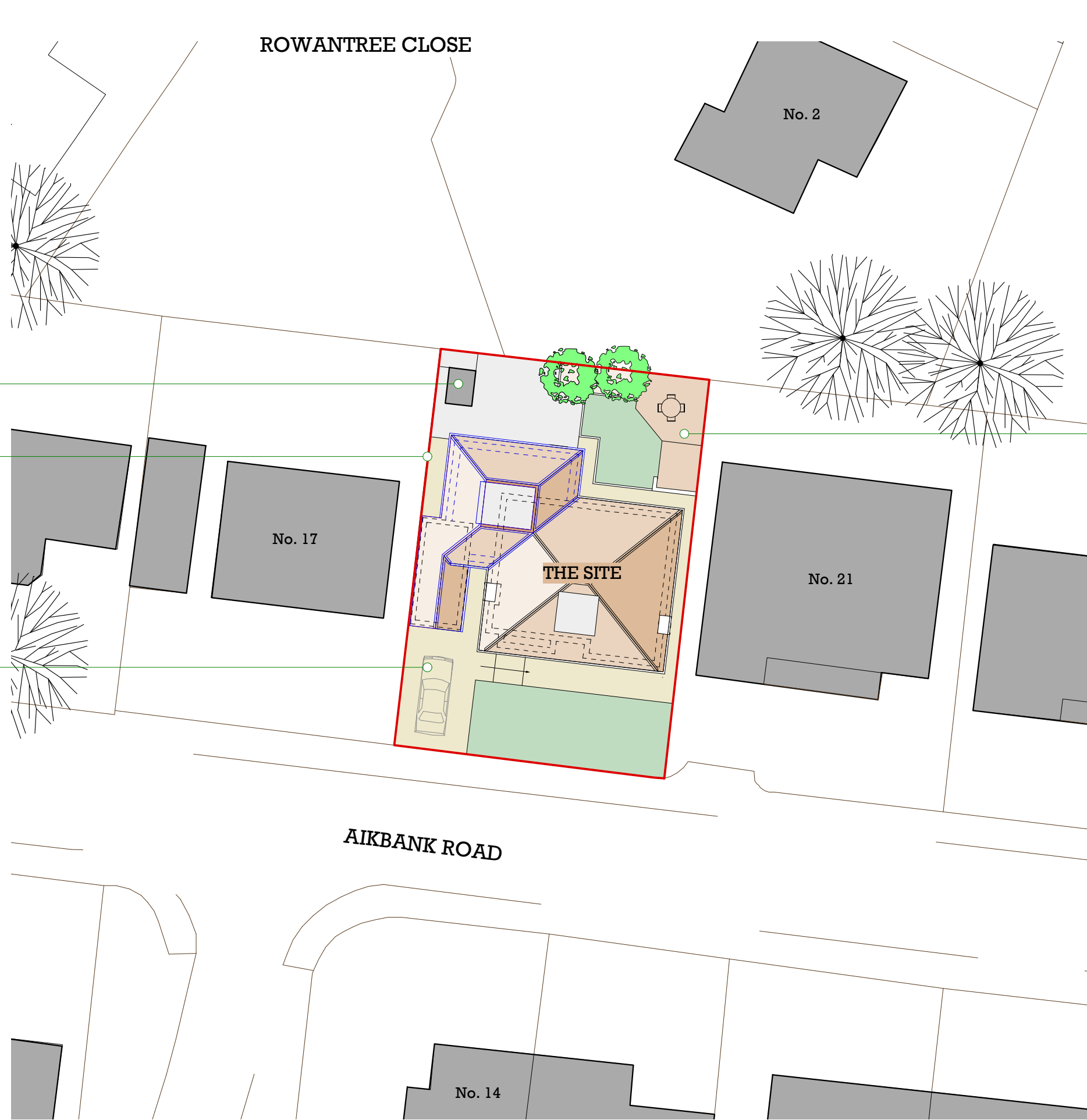
1 PLAN - PROPOSED SITE SCALE 1:250 @ A3
