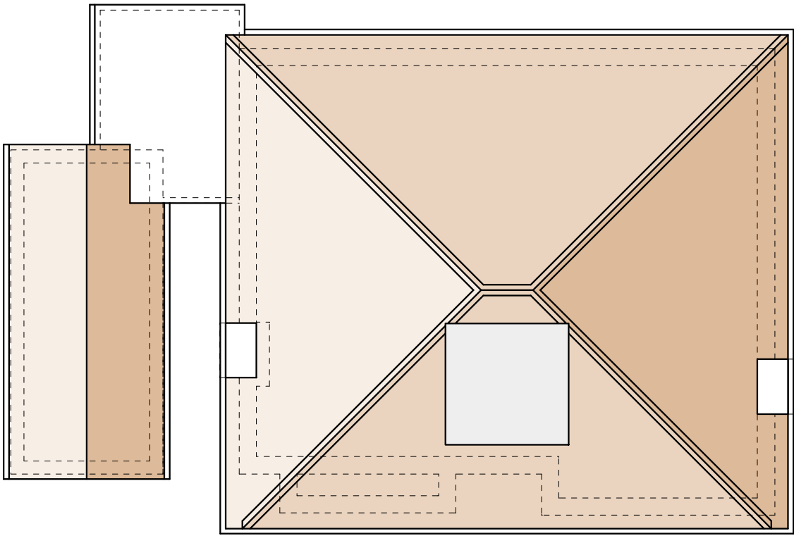
2 PLAN - EXISTING ROOF SCALE 1:100 @ A3
