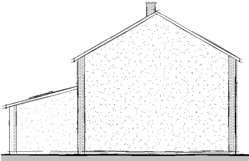
Side Elevation 02
