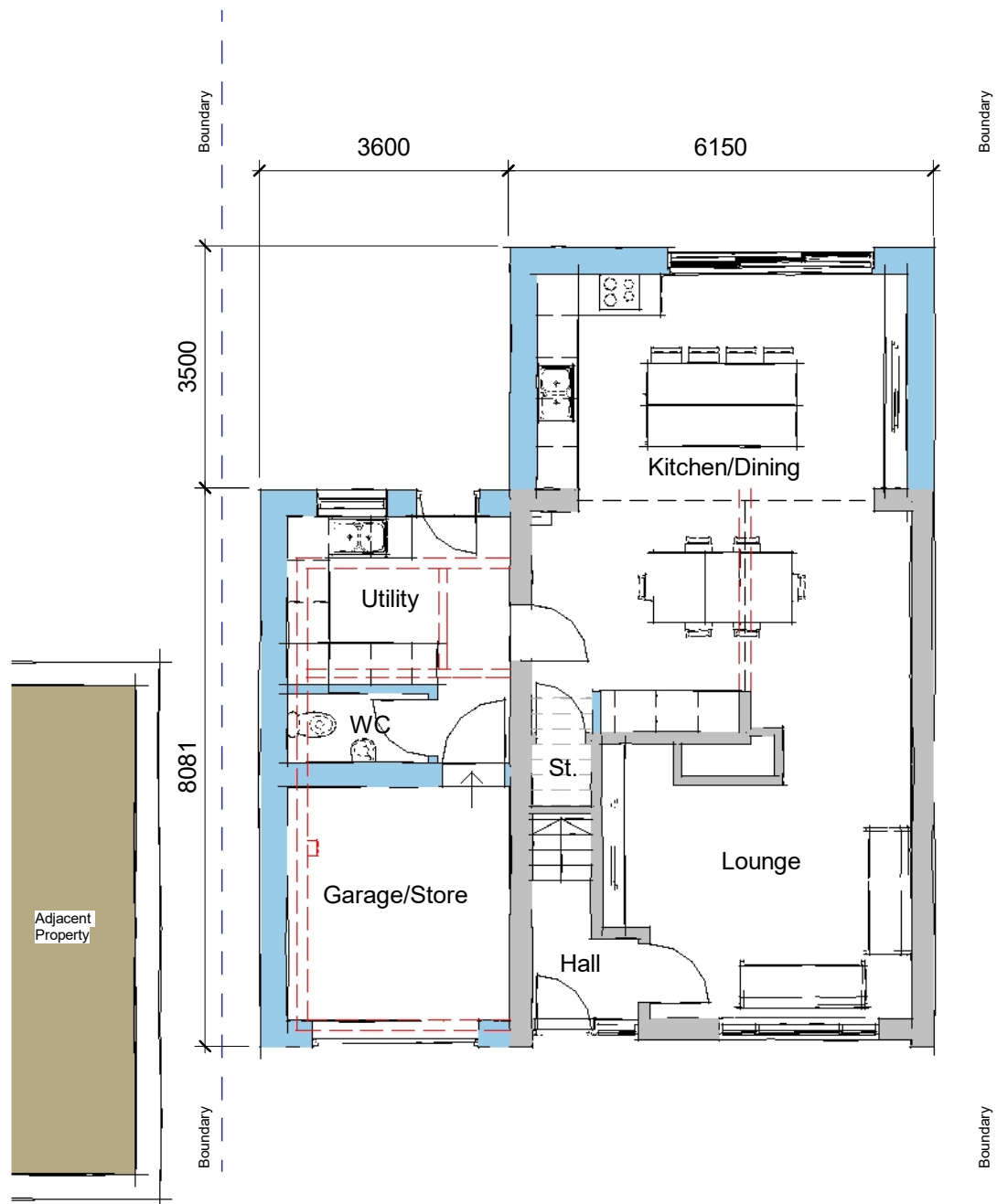
Ground 1 : 100
