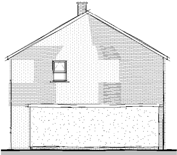
Side Elevation 02 1 : 100
