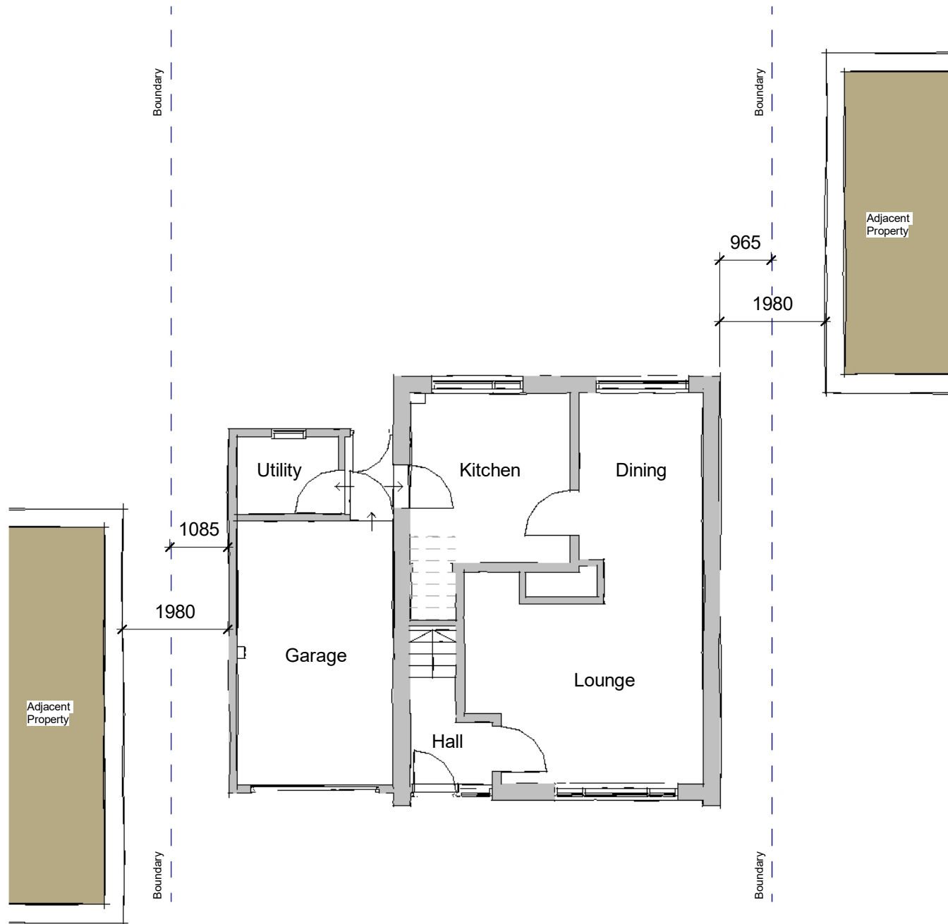
Ground 1 : 100
