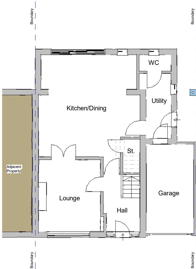
Ground 1 : 100
