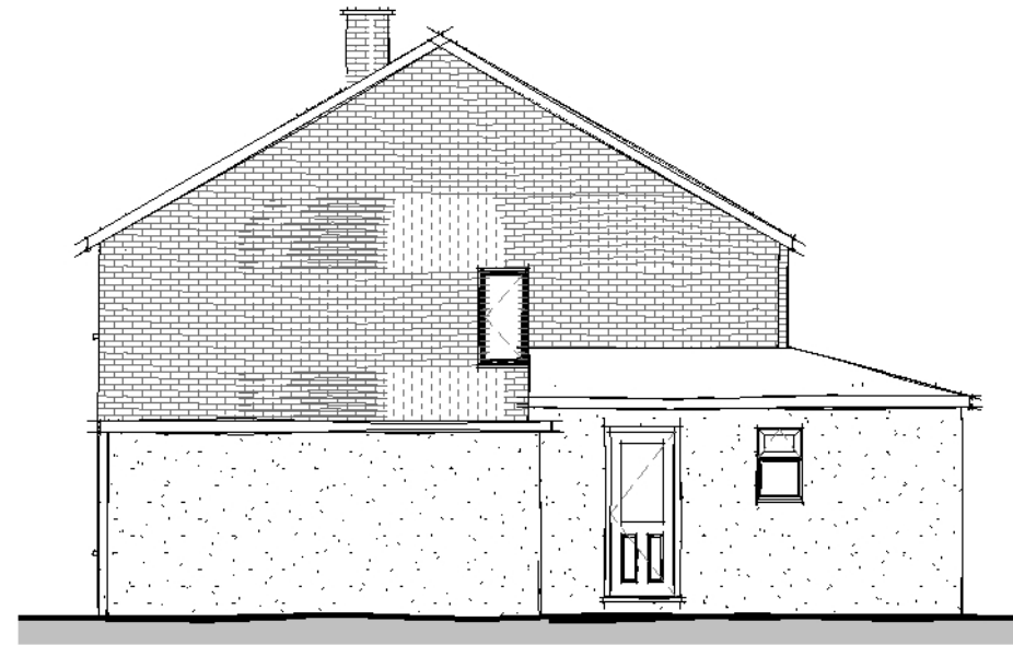
Side Elevation 01
