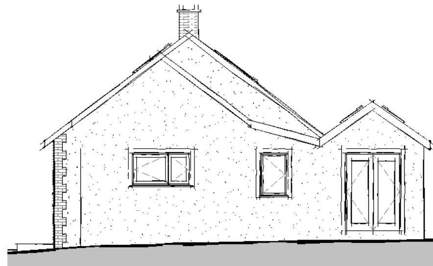
Rear Elevation 1 : 100
