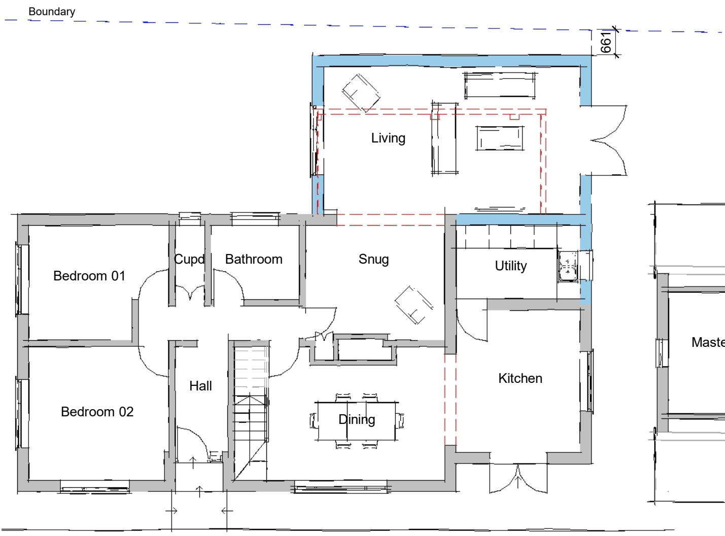
Ground 1 : 100
