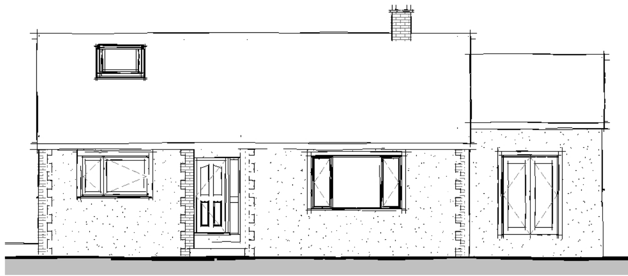
Side Elevation 02 1 : 100
