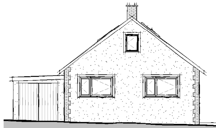
Front Elevation 1 : 100
