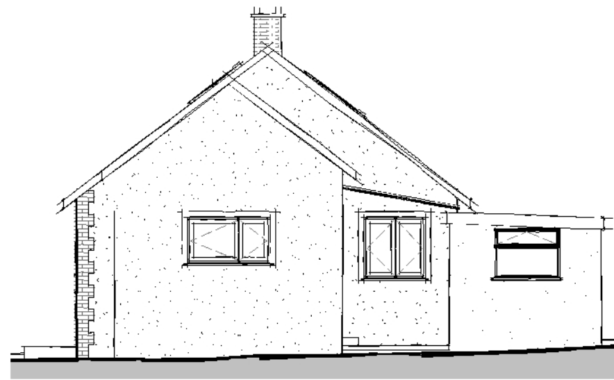
Rear Elevation 1 : 100
