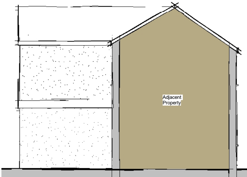
Side Elevation 02 1 : 100
