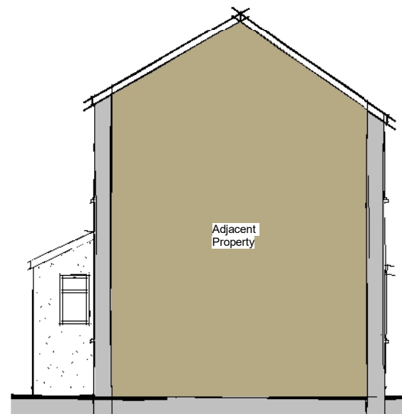
Side Elevation 02 1 : 100
