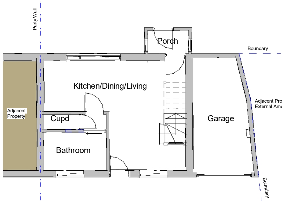
Ground 1 : 100
