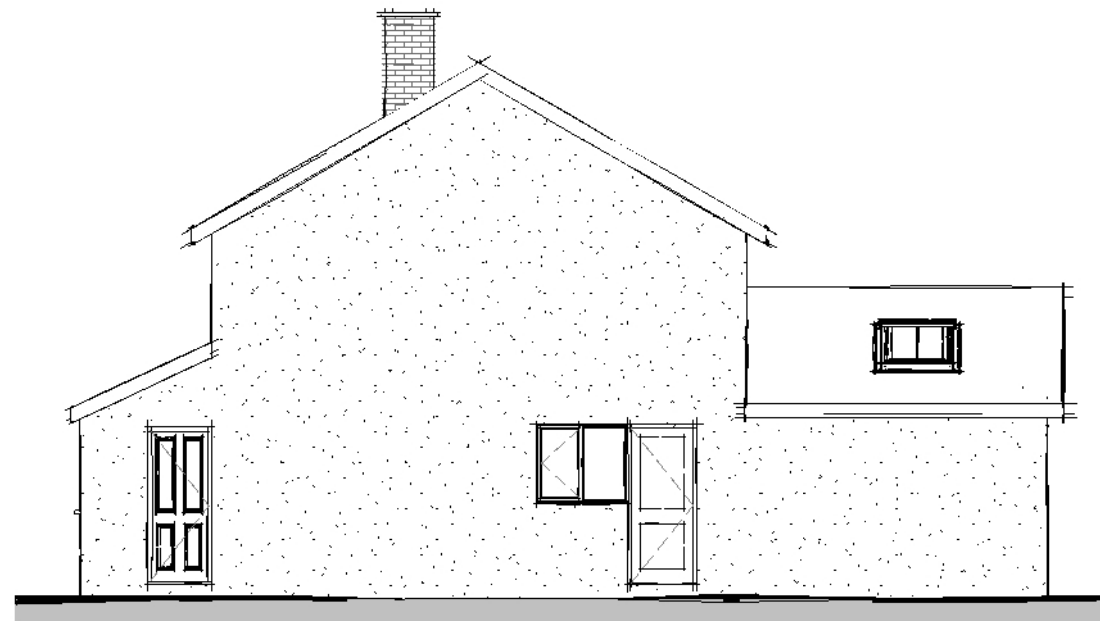
Side Elevation 01
