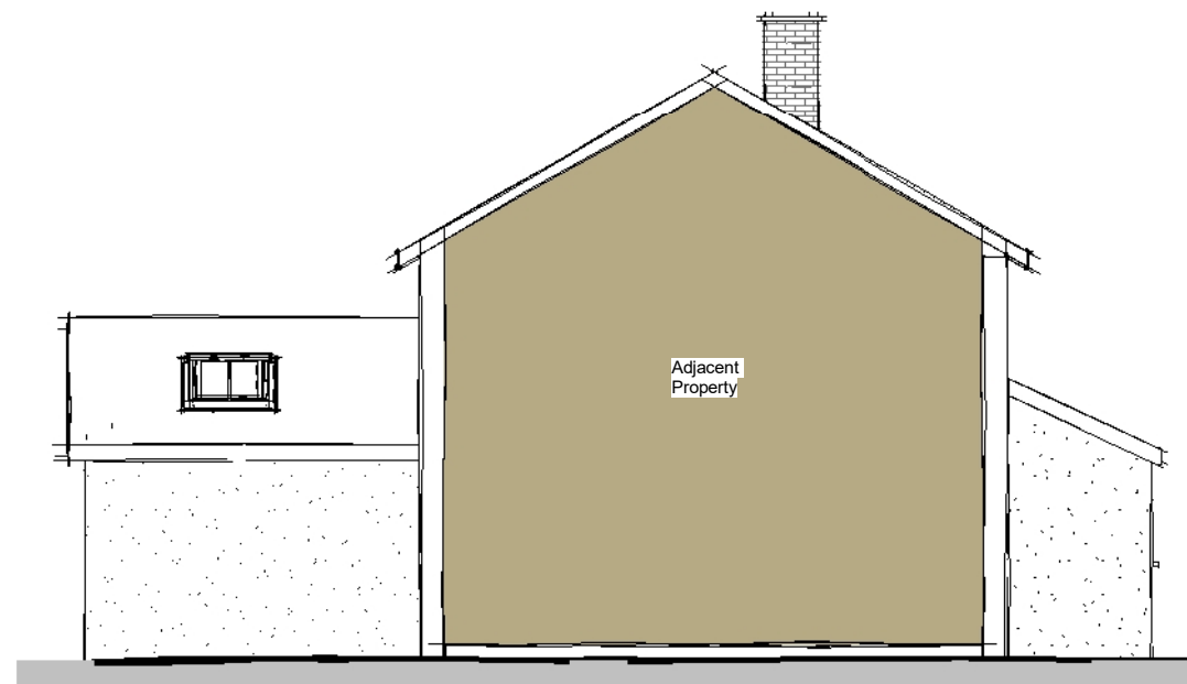
Side Elevation 02
