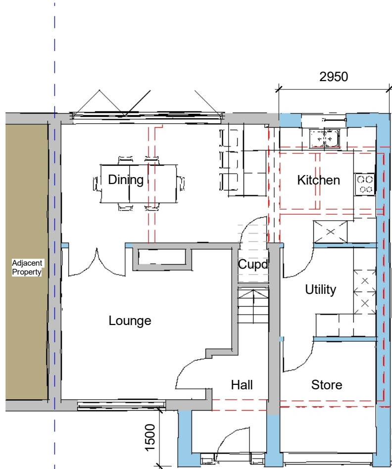
Ground 1 : 100
