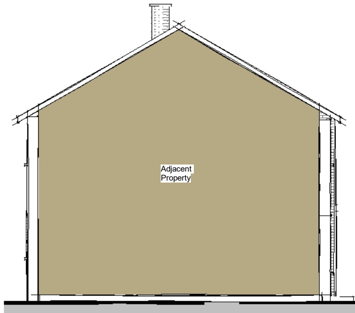
Side Elevation 02 1 : 100
