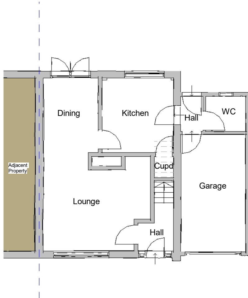
Ground 1 : 100
