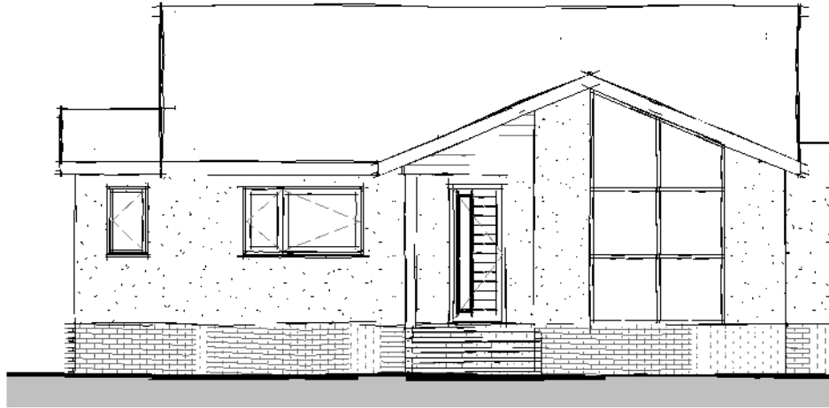
Front Elevation 1 : 100
