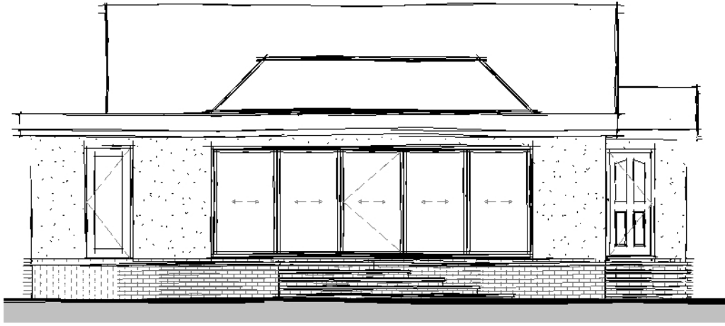
Rear Elevation 1 : 100
