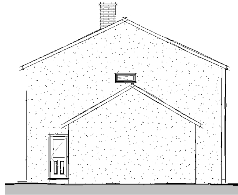
Side Elevation 02
